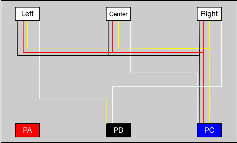
Ultrasonic Harness
