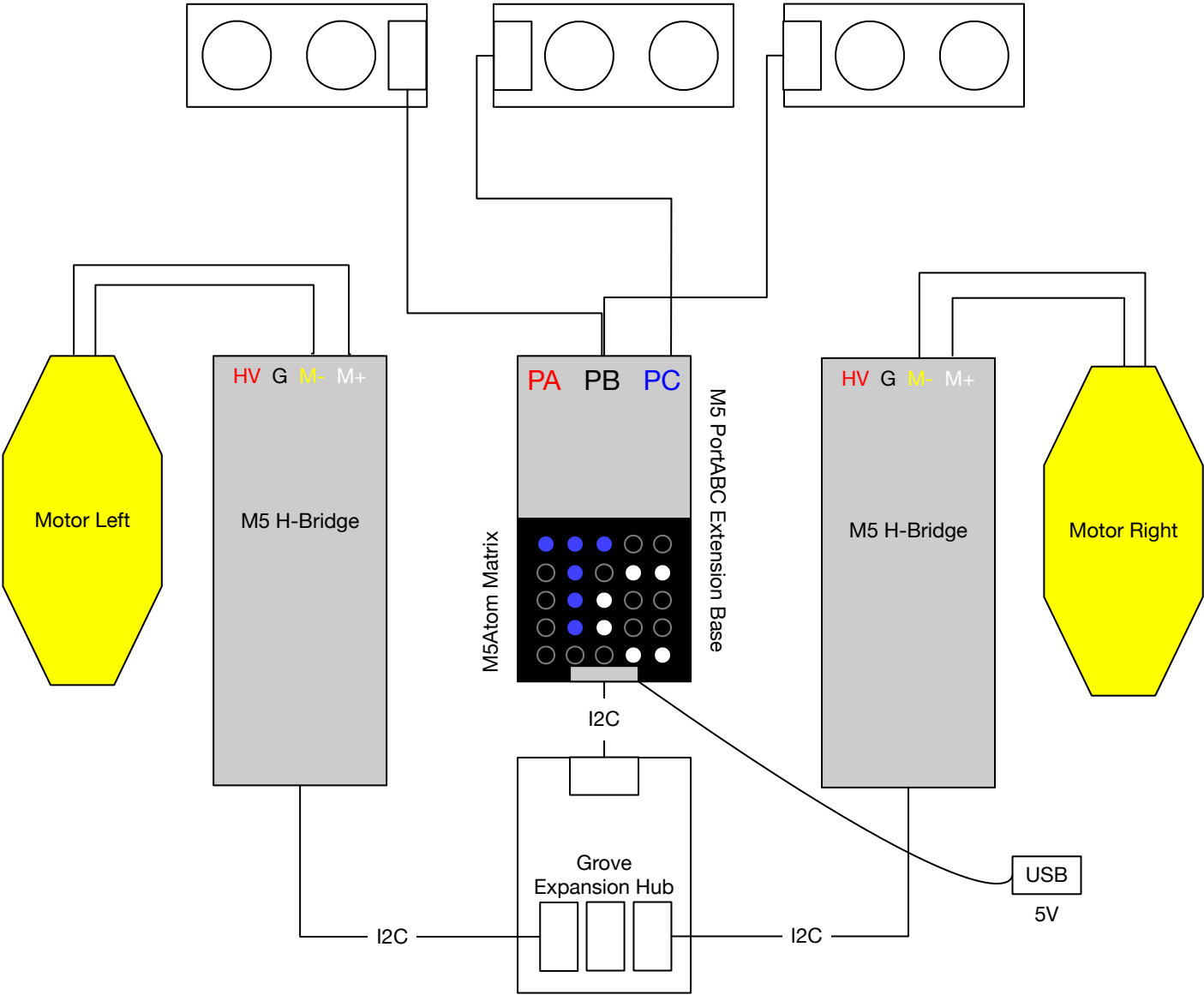
Ultrasonic Harness
